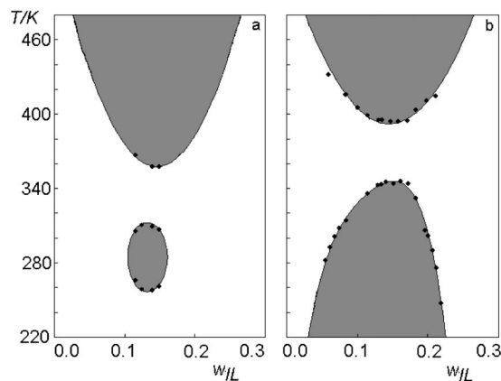
FIGURE 9. Fluid T -composition phase diagrams of quasi-binary mixtures of (a) [(C_4mim)[NTf_2]] plus [(C_5mim)[NTf_2]] plus CHCl_3 and (b) [(C_5mim)[NTf_2]] plus (CHCl_3 plus CCl_4) , in which the two-phase regions correspond to the shaded areas. The two pseudocomponents have a composition ratio corresponding to [C_{4.33}mim][NTf_2] in a and CH_{0.94}Cl_{3.06} in b.
